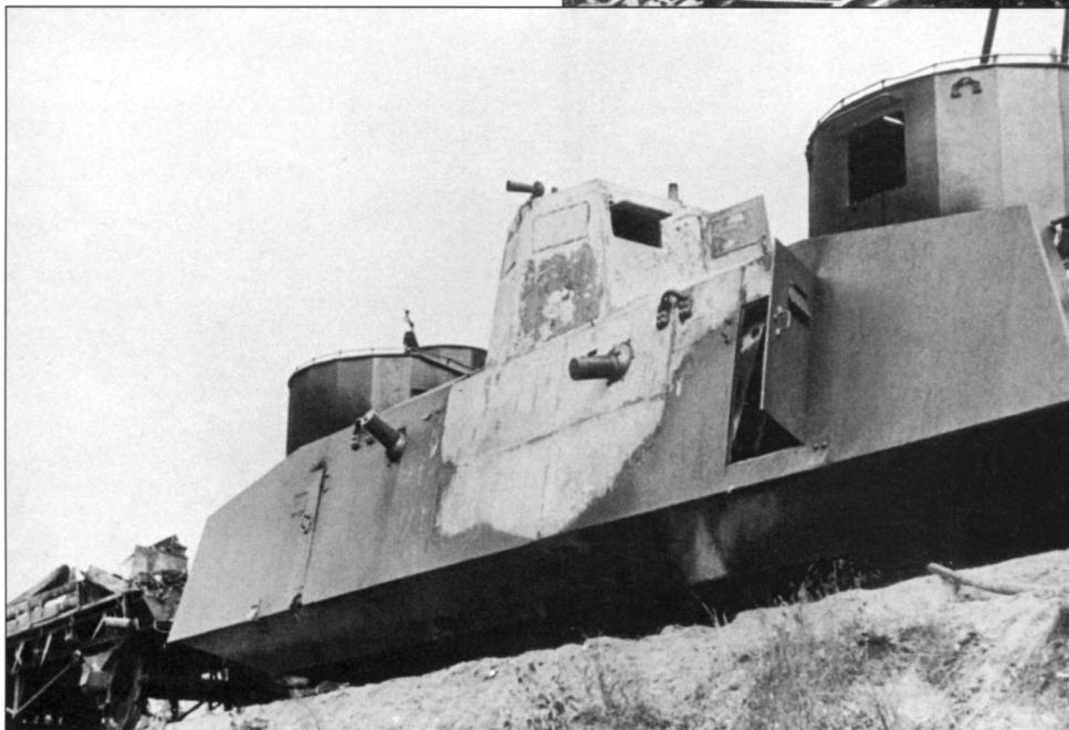
This battle-wagon of a Soviet armored train was burned out after receiving a direct hit, probably courtesy of the Luftwaffe. The light color on the central part of the armor is an indication of the intense heat of the fire.
