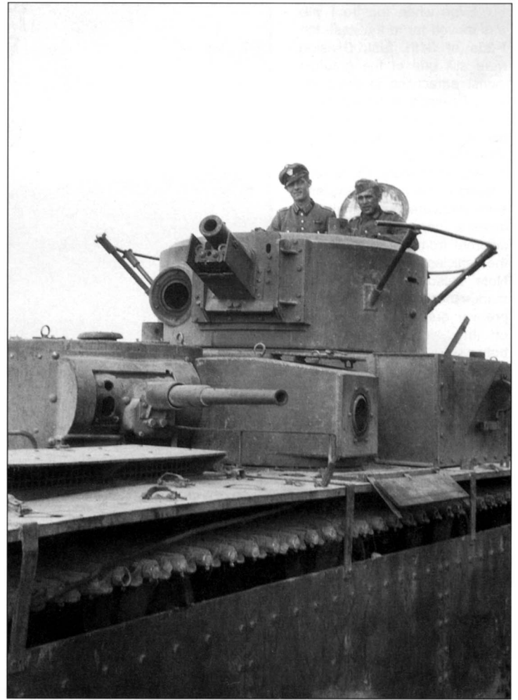
Close-up view of a T-35 tank with its German captors posing in the main turret. Note that the tracks are still on the vehicle. Just visible at the bottom right-hand corner of the photo is the red star national insignia. Note the many details of the turret construction.
