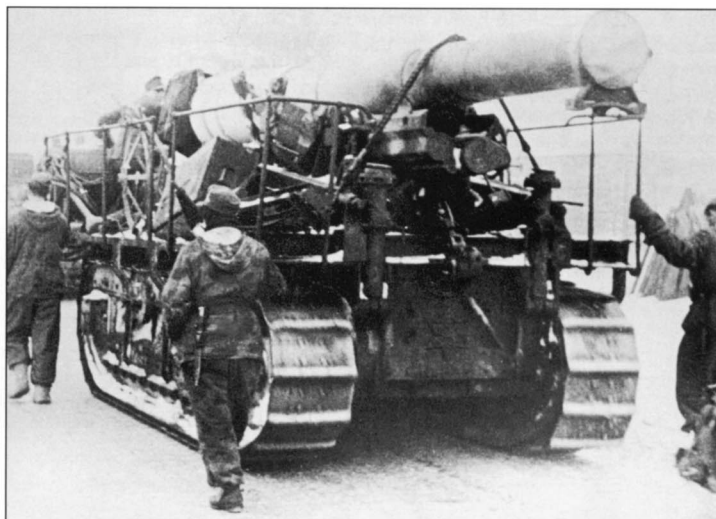
In 1942 the 194mm Kanone 485(f), the old French self-propelled gun produced in the mid-1930s, was sent into action in the northern sector of the Eastern Front for use in the siege of Leningrad. The vehicle is probably painted with French camouflage.
