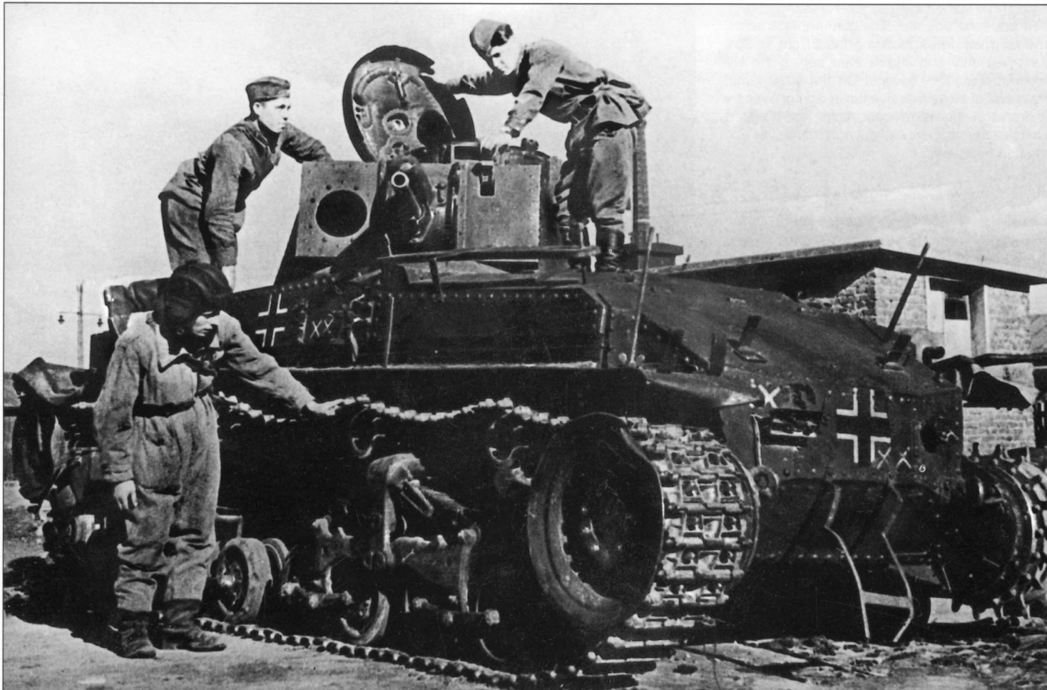
Soviet soldiers inspect a captured Pz.Kpfw. 35(t) from 6.Panzer-Division. Note the divisional markings — XX — on the side of superstructure, as well as another set on the rear hull plate. By the end of August 1941, 6.Panzer-Division had lost 35 tanks, and another 33 had been damaged. By the winter of 1941/42, almost all of the division's tanks had been lost in the fields or forests of northern Russia, mainly due to breakdowns.
